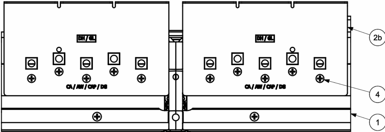
TOP VIEW - SPLIT MULL GUSSET PLATE SCALE 1 : 2
