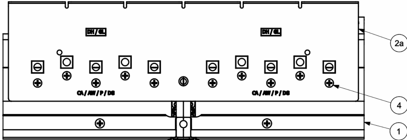
TOP VIEW - FULL GUSSET PLATE SCALE 1 : 2
